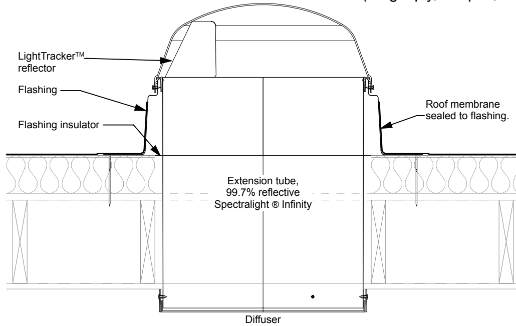
SECTION INSULATION OVER JOISTS
